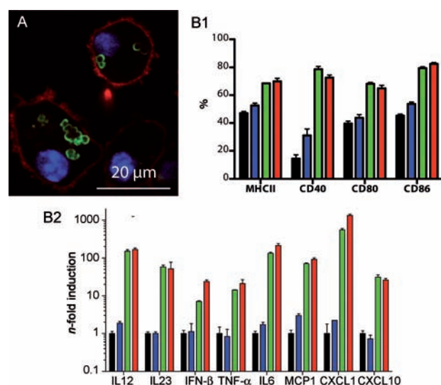
Figure 2. A) Confocal microscopy image of DCs that internalized (\text{DS}/\text{pLArg})_2 capsules coated with fluorescein isothiocyanate (FITC)-labeled CpG-containing oligos (green). The cell membrane was stained with cholera toxin subunit B conjugated to Alexa Fluor 647 (red) and cell nuclei with 4',6-diamidino-2-phenylindole (DAPI, blue). B1) Flow-cytometric analysis of DC maturation. Graphs show the percentages of DCs high in the expression of MHCII, CD40, CD80, and CD86 in the presence of phosphate-buffered saline (PBS, black), capsules (blue), CpG-containing oligos in solution (green), and capsules functionalized with CpG-containing oligos (red); B2) real-time quantitative PCR analysis of the expression of polarizing cytokines (IL-12, IL-23, and IFN- \beta ), pro-inflammatory cytokines (IL-6 and TNF- \alpha ), and inflammatory chemokines (MCP-1, CXCL-1, and CXCL-10) after a 12 h incubation period of bone-marrow-derived DCs in the presence of the reagents listed under (B1); also the same color code applies. Note that in all experiments (in solution and on the functionalized capsules) equal amounts of CpG-containing oligonucleotides were used.
